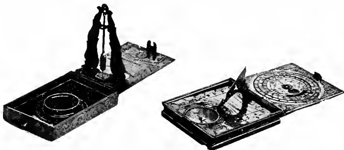
Two Gilt-brass Portable Dials, 1578, 1553.
